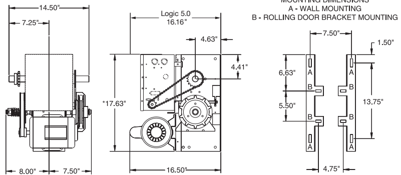
*FOR MODELS WITH BRAKES, ADD 2" (BRAKE STANDARD ON 3/4 AND 1 HP, OPTIONAL ON 1/2 HP)
